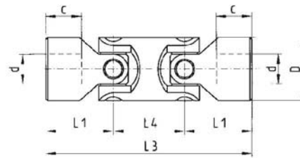
Precision single joint GD
